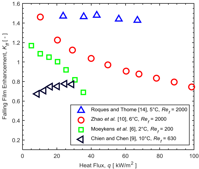
Fig. 1. Comparison of literature values for falling film enhancement factor K_{ff} for plain tubes for R-134a at saturation temperatures close to 5 °C.
