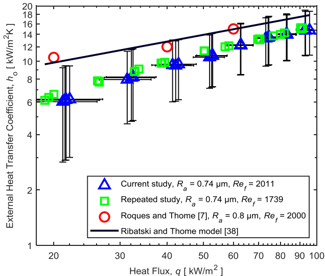
Fig. 11. Falling film boiling on a copper tube at a saturation temperature of 5 °C.
