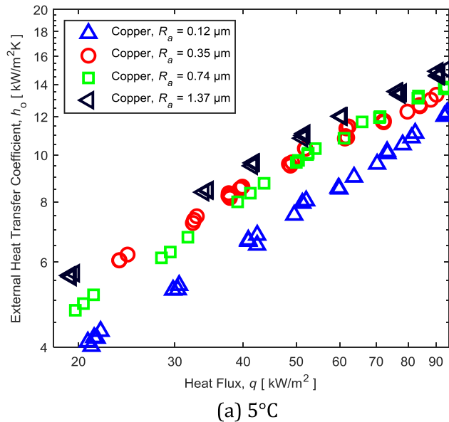
Fig. 12. Pool boiling with different roughnesses of copper tube at different saturation temperatures.
