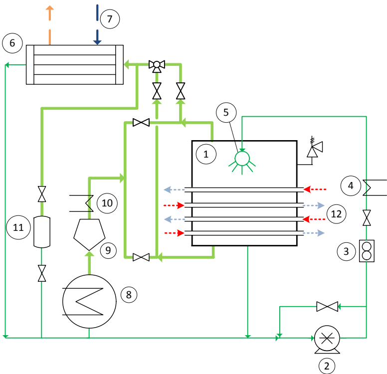
Fig. 2. Schematic of refrigerant loop.
