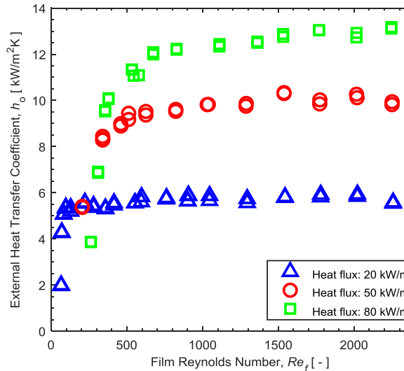
(b) R_a of 0.74 \mu\text{m}
