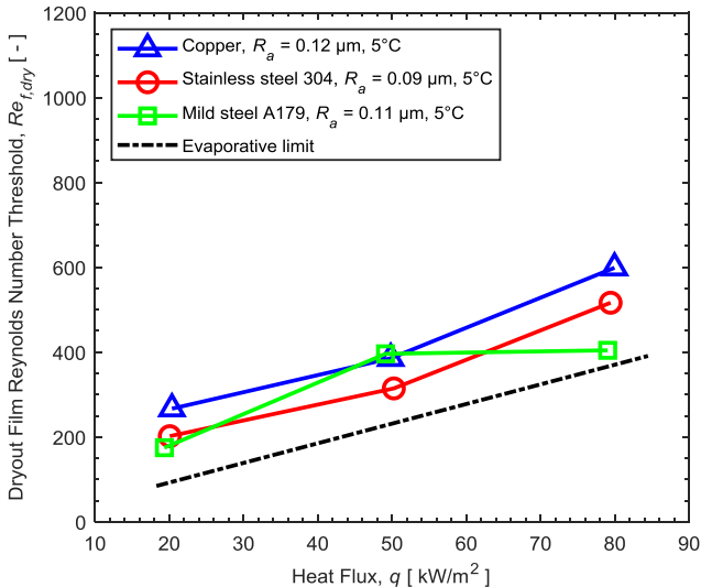
Fig. 22. Total dryout threshold Re_{f,dry} as a function of heat flux for different material tubes at a saturation temperature of 5^\circ\text{C} .
