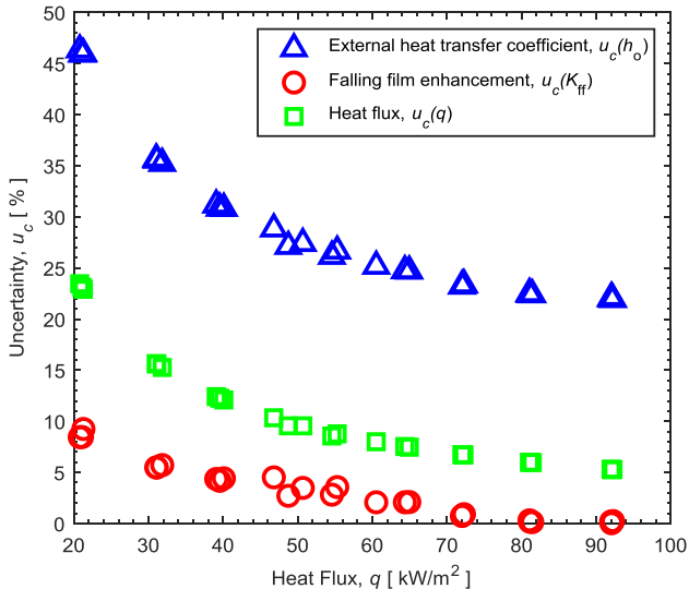
Fig. 8. Uncertainties as a function of heat flux at 5 °C for a copper tube under falling film boiling conditions with a R_a of 0.12 \mu\text{m} .
