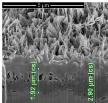
(f) CuO – cross-section
