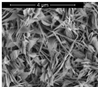
(e) CuO – top view
