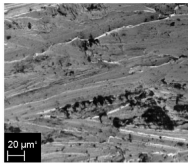
(b) Roughened
