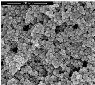
(c) LbL – top view
