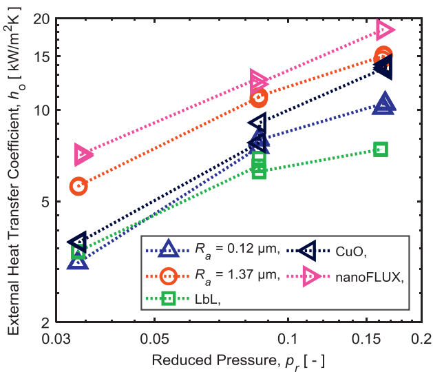
Fig. 7. HTC's of surfaces as a function of reduced pressure at 50 \text{ kW/m}^2 .
