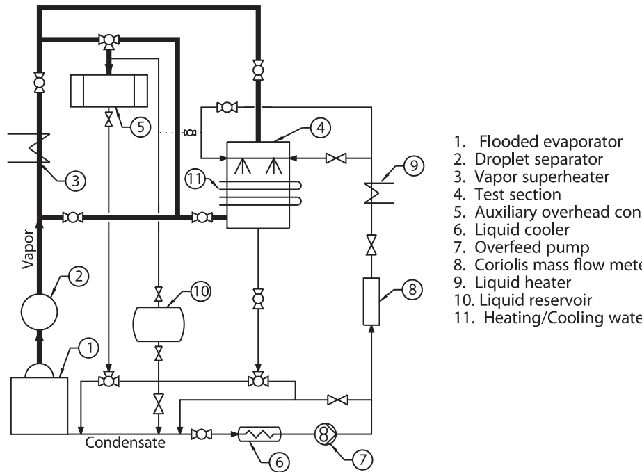
Fig. 1 – Schematic of the refrigerant circuit in the Falling Film Facility.
