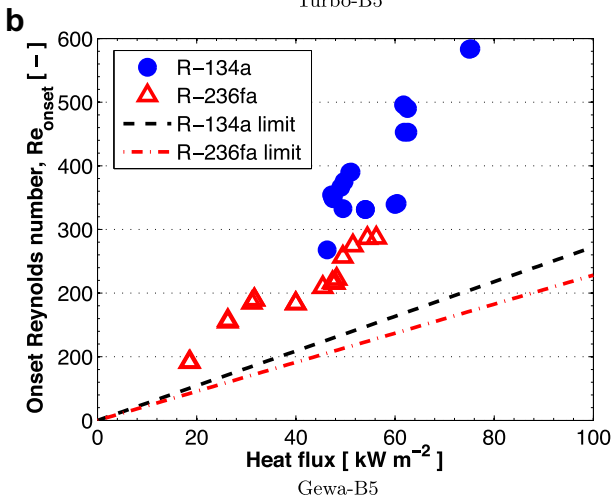
Fig. 10 – Onset-of-dryout Reynolds numbers for the enhanced tubes of the current study.
