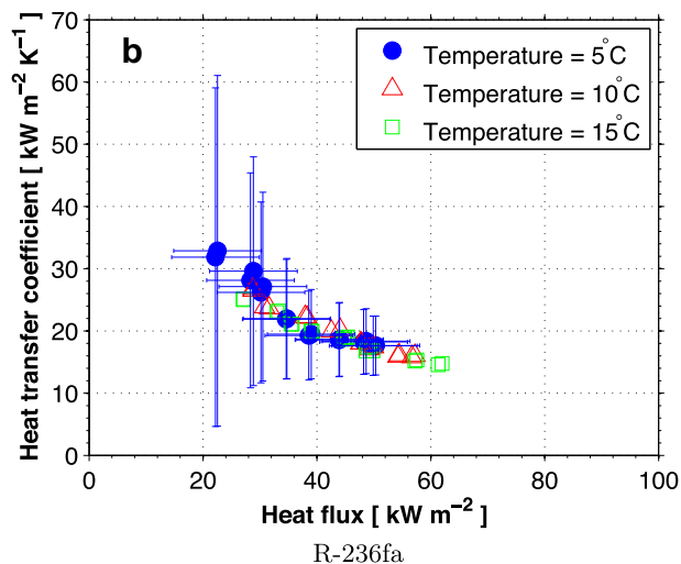
Fig. 3 – Pool boiling measurements on tube Gewa-B5.
