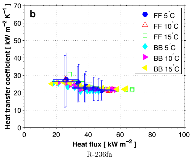
Fig. 4 – Comparison of pool boiling measurements on tube Turbo-B5 performed on the LTCM's falling film and bundle boiling facilities.
