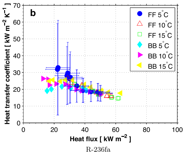
Fig. 5 – Comparison of pool boiling measurements on tube Gewa-B5 performed on the LTCM's falling film and bundle boiling facilities.
