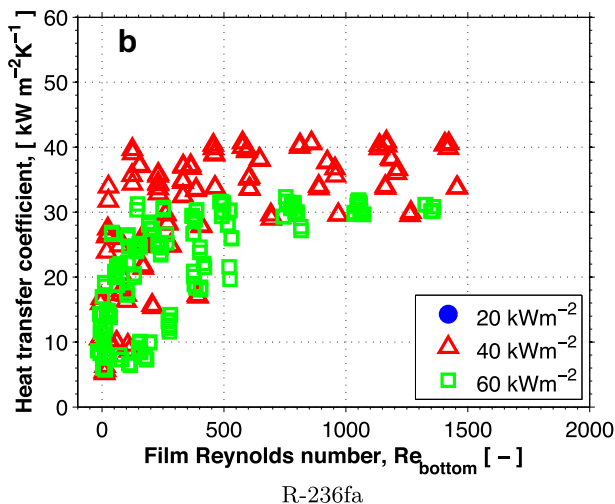
Fig. 7 – Falling film evaporation on a Gewa-B5 tube bundle and single array at T_{\text{sat}} = 5\text{ }^{\circ}\text{C} .
