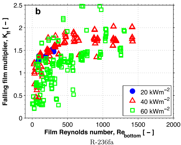
Fig. 8 – Falling film multiplier for the Turbo-B5 tube bundle and single array at T_{sat} = 5\text{ }^{\circ}\text{C} .
