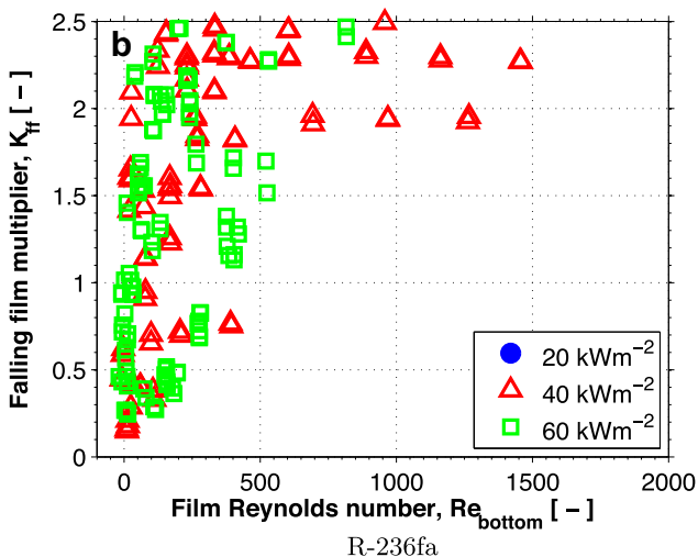
Fig. 9 – Falling film multiplier for the Gewa-B5 tube bundle and single array at T_{sat} = 5^\circ\text{C} .
