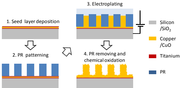
Figure 1: CuO hierarchical surfaces were fabricated as follows: (1) Ti/Cu/Ti layers were deposited on a silicon substrate. (2) A thick ( \approx 100\ \mu\text{m} ) PR mold was patterned using photolithography. (3) The top Ti layer was removed to expose the Cu layer and then Cu micropillars were electroplated. (4) After removing the photoresist, Cu micropillars were oxidized in an alkali solution composed of \text{NaClO}_2 , \text{NaOH} , \text{Na}_3\text{PO}_4 \cdot 12\text{H}_2\text{O} to form CuO nanostructures.
