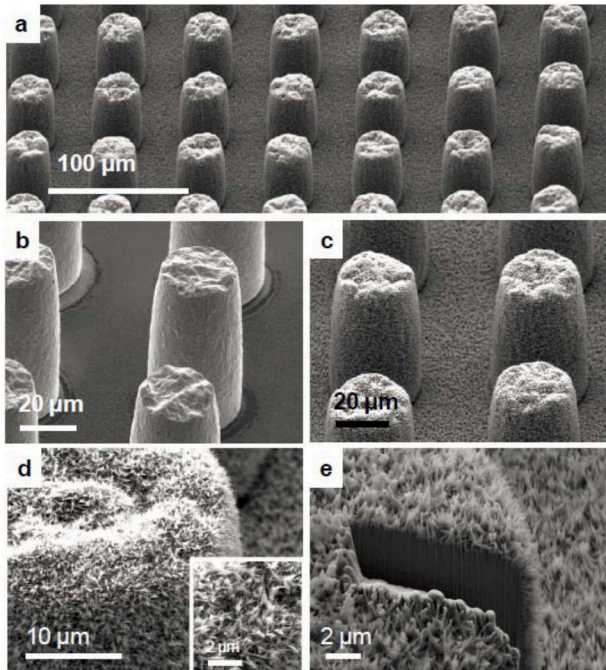
Figure 2: Scanning electron micrographs (SEMs) of the representative, fabricated CuO-based hierarchical surfaces. (a) CuO micropillar array in a square array with heights of 61 μm, diameters of 30 μm, and spacings of 30 μm. (b) Electroplated Cu micropillars, and (c) micropillars with CuO nanostructures formed on the surfaces. (d) Magnified view of the CuO micropillar and CuO nanostructures formed on the surfaces (inset). (e) Cross-sectional view of the CuO micropillar obtained using FIB milling.
