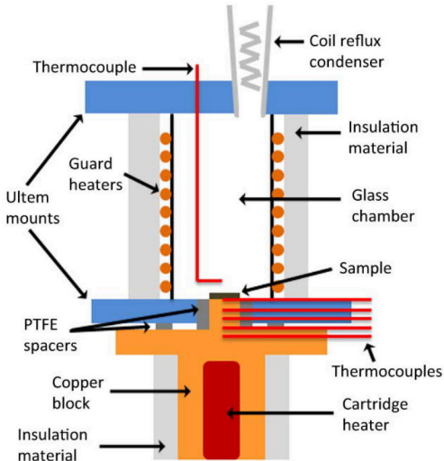
Figure 3: Schematic of the experimental pool boiling setup [12]. The setup consists of a copper block and a glass chamber fixed at both ends by Ultem mounts. Cartridge heaters were imbedded in the copper block allowing for a maximum power of 1400 W. Five in-line thermocouples were inserted into the center axis of the copper block to measure the heat flux and surface temperature.
