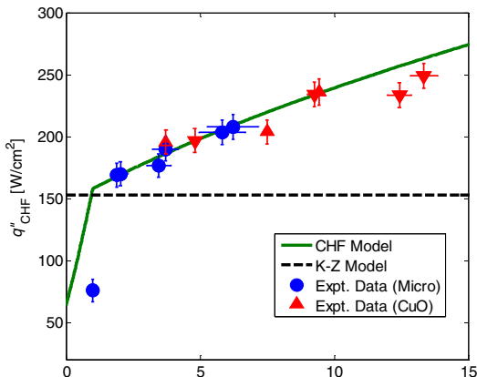
Figure 5. CHF as function of \alpha ( = r \cos \theta_{rec} ). The proposed model (solid line) is compared to the K-Z model with a factor of K = 0.18 (dashed line). The symbols show the CHF data for (●) microstructured surfaces [12], and (▼) CuO hierarchical surfaces, as a function of the estimated \alpha values.
