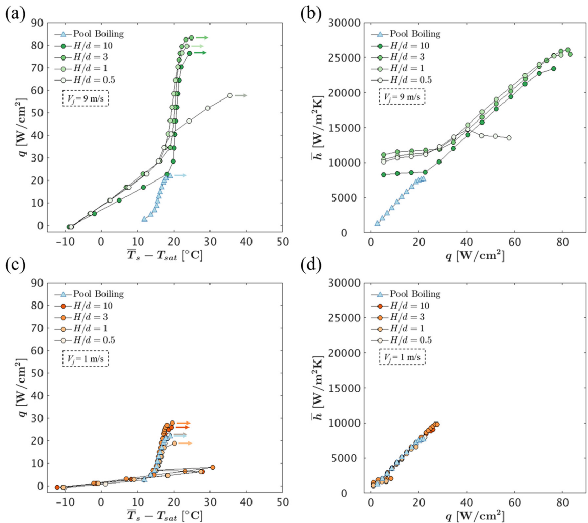
Fig. 3. (a and c) Boiling curves and (b and d) heat transfer coefficients as a function of heat flux for the jet impingement configuration (corresponding to V_j = 9 \text{ m/s} and 1 \text{ m/s} , respectively; H/d = 0.5, 1, 3 , and 10 ) compared with pool boiling.
