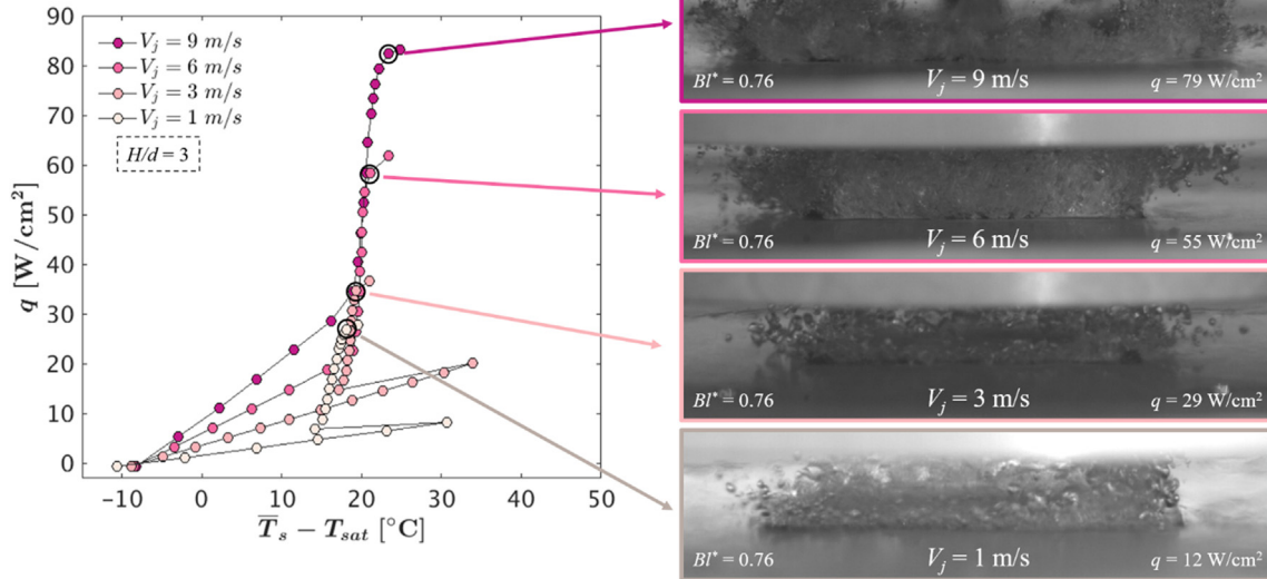
Fig. 5. Comparison of high-speed video frames across four jet velocities ( V_j = 1 m/s, 3 m/s, 6 m/s, and 9 m/s; H/d = 3 ) at a constant non-dimensional heat input ( Bl^* = 0.76 ). The corresponding heat fluxes for each jet velocity are highlighted on the boiling curve. Full videos are included in the Supplementary Materials .
