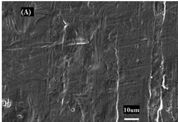
Fig. 2. SEM images of the (A) bare copper surface and (B) sand blasted copper.
