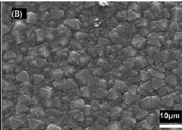
Fig. 3. EM images of diamond coating on the (A) bare copper surface and (B) sand blasted copper.
