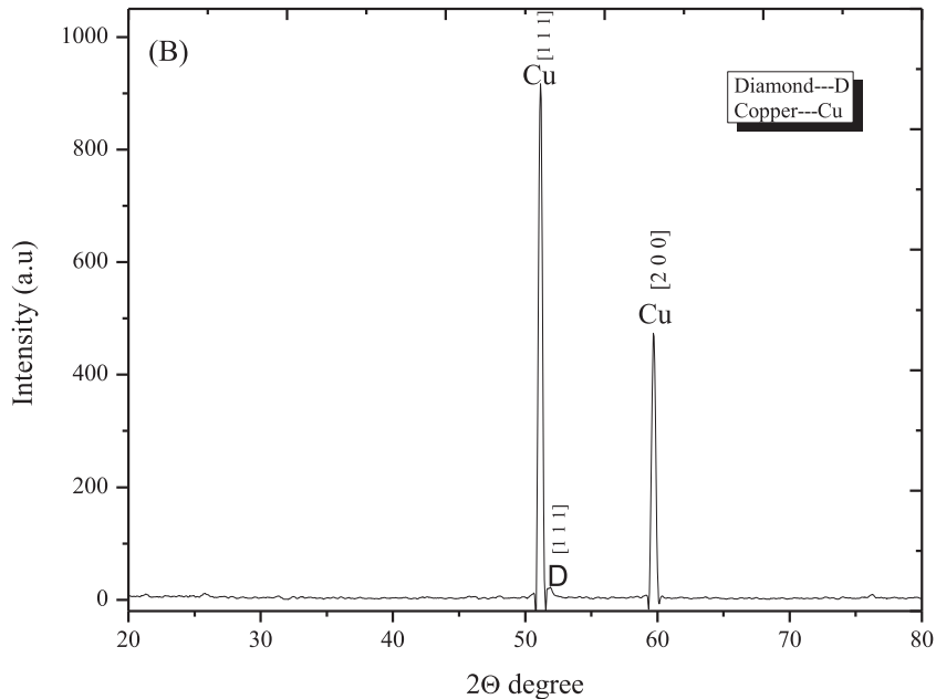
Fig. 4. XRD patterns of the diamond coating on (A) untreated copper and (B) sandblasted copper.
