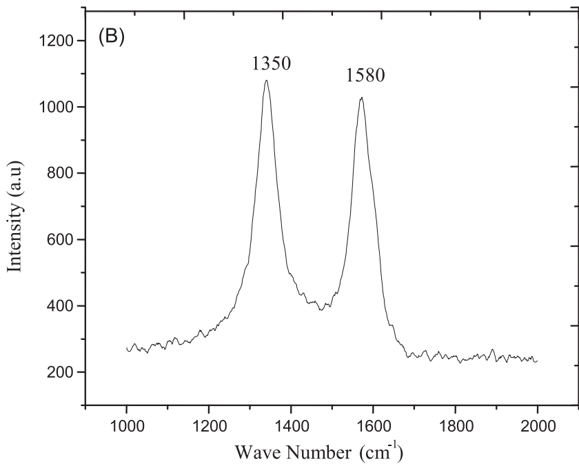
Fig. 6. Raman spectrum of (A) diamond coating on sand blasted Cu. (B) CNT coating on the diamond coated Cu.
