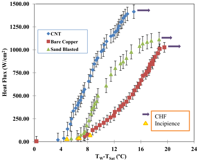
Fig. 8. Pool boiling curve for different surfaces.
