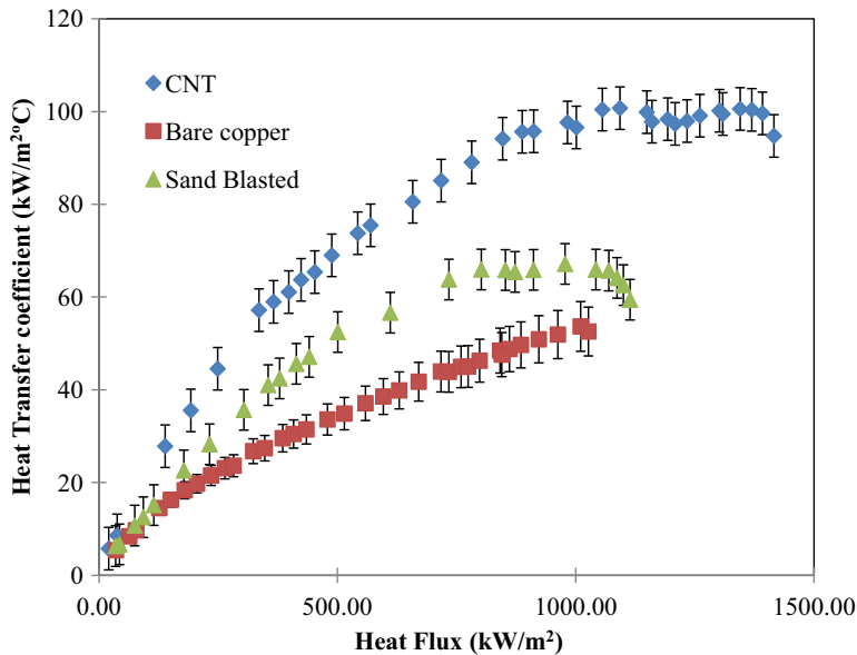
Fig. 9. Variation of the boiling heat transfer coefficient for different surfaces.
