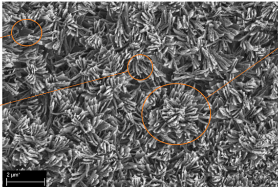
Fig. 2–3. Nanostructure identification on SEM photograph of CuO nanocoated copper sample.
