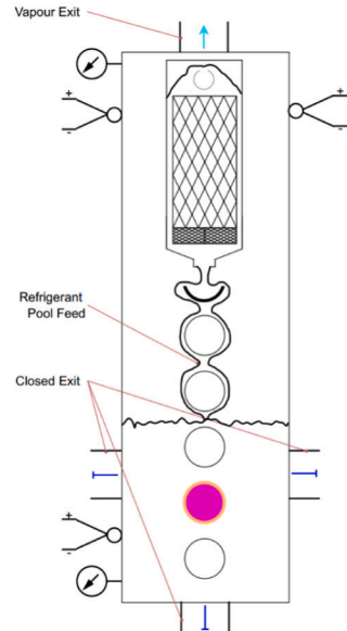
(b) Test chamber
