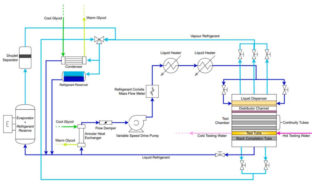
(a) Refrigerant circuit
