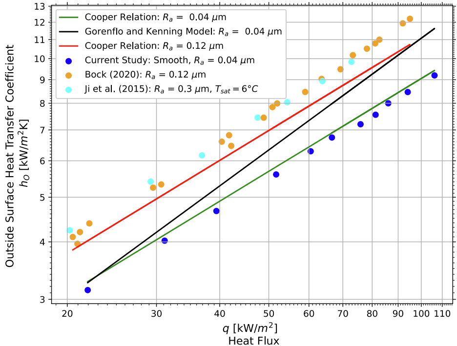
Fig. 3–1. Smooth tube pool boiling validation test in R134a at 5^\circ\text{C} .
