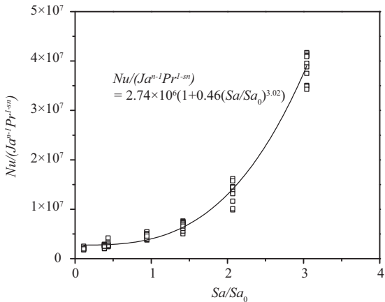
Fig. 12. Evaluation of C by plotting Nu/Ja^{n-1}Pr^{1-sn} as a function of Sa/Sa_0 .
