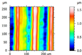
(b) Waviness (long-scale component)
