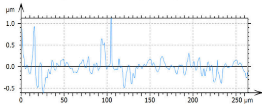
(c) Roughness (short-scale component)
