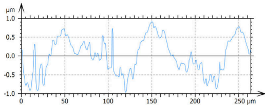
(b) Waviness (long-scale component)
