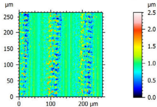
(c) Roughness (short-scale component)
