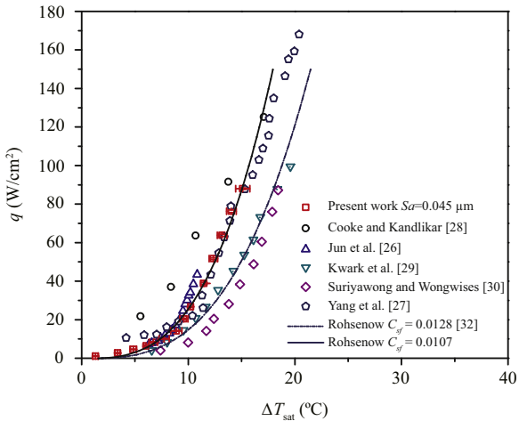
Fig. 6. Comparison of present experimental data with those in previous literature and Rohsenow correlation.
