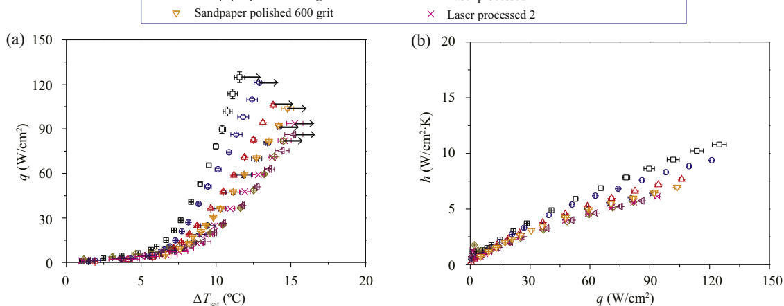
Fig. 7. Pool boiling curves of all the testing surfaces, (a) heat flux q as a function of wall superheat \Delta T_{sat} , (b) heat transfer coefficient h as a function of heat flux q .
