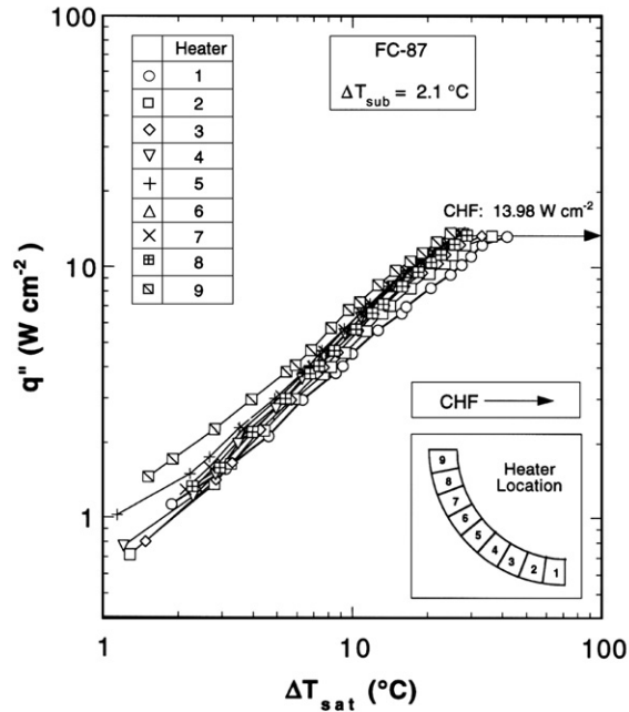
Fig. 3. (a) Local boiling curves for nine heaters. (b) Transient heater temperatures following CHF.
