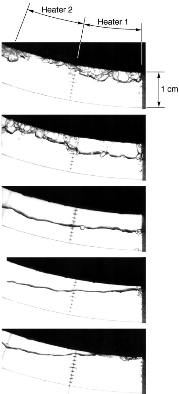
Fig. 6. Development of vapor layer for heaters 1 and 2 at CHF-.
