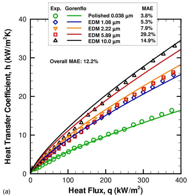
Fig. 11 Comparison between experimental data and predictions from the Gorenflo correlation [34] for (a) water and (b) FC-77
