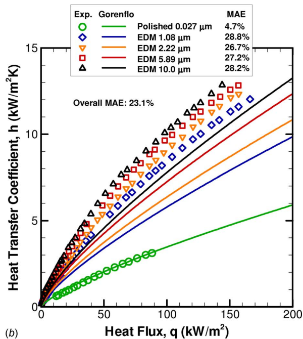
Fig. 11 Comparison between experimental data and predictions from the Gorenflo correlation [34] for (a) water and (b) FC-77
