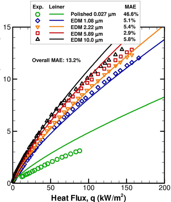
Fig. 12 Comparison between experimental data and predictions from the Leiner correlation [59] for (a) water and (b) FC-77
