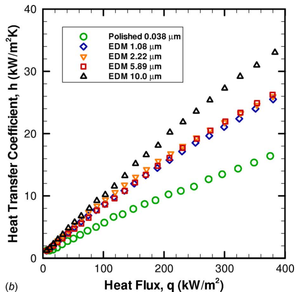
Fig. 3 Boiling curves for water: (a) heat flux versus wall superheat and (b) heat transfer coefficient versus heat flux
