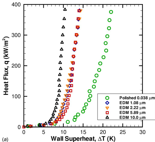
Fig. 3 Boiling curves for water: (a) heat flux versus wall superheat and (b) heat transfer coefficient versus heat flux
