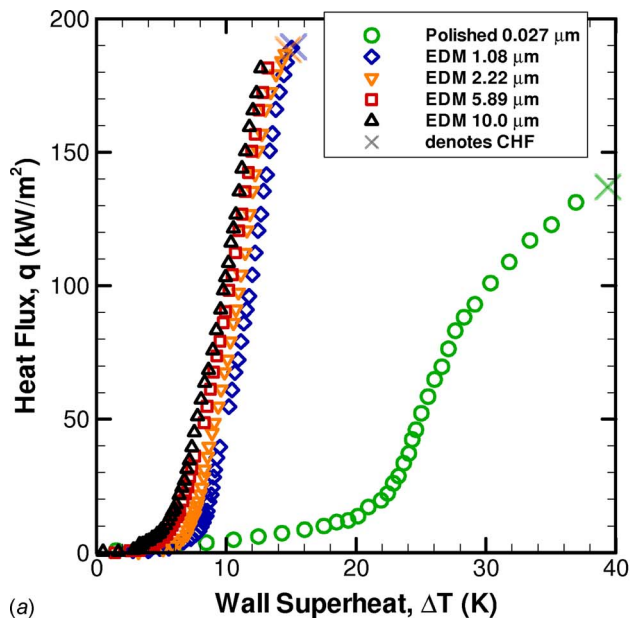
Fig. 4 Boiling curves for FC-77: (a) heat flux versus wall superheat and (b) heat transfer coefficient versus heat flux
