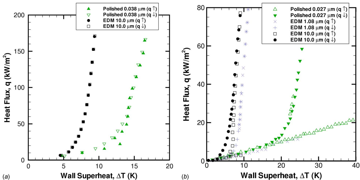
Fig. 5 Boiling curves showing the hysteresis effect for (a) water and (b) FC-77, where q \uparrow indicates data obtained in order of increasing heat flux and q \downarrow indicates those in order of decreasing heat flux. It is noted that a smaller heat flux increment was used experimentally than is indicated in (b); only a fraction of the data are included to improve readability of the figure.
