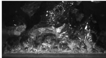
Fig. 6 Photographs of the boiling process in water for varying heat flux and surface roughness. The physical width of each image is approximately 25 mm.
