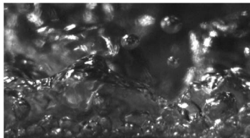
Fig. 7 Photographs of the boiling process in FC-77 for varying heat flux and surface roughness. The physical width of each image is approximately 7.3 mm.
