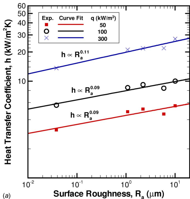
Fig. 8 Dependence of heat transfer coefficient on surface roughness for (a) water and (b) FC-77. The solid lines represent a curve fit through all five experimental data points (one polished surface and four EDM surfaces). The dashed lines in (b) represent a curve fit to only the four EDM surfaces (excluding the 0.027 μm polished surface).
