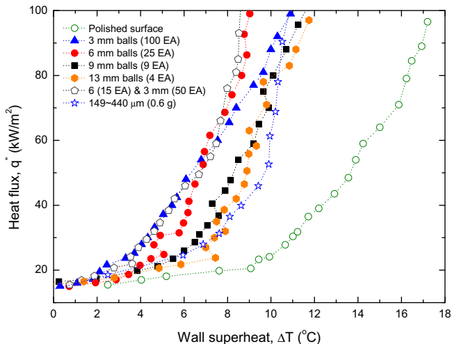
Fig. 4. Boiling curve showing the effect of the free particle size on boiling heat transfer. The experimental results for 10 \mu m and 20–40 nm particles are not shown.
