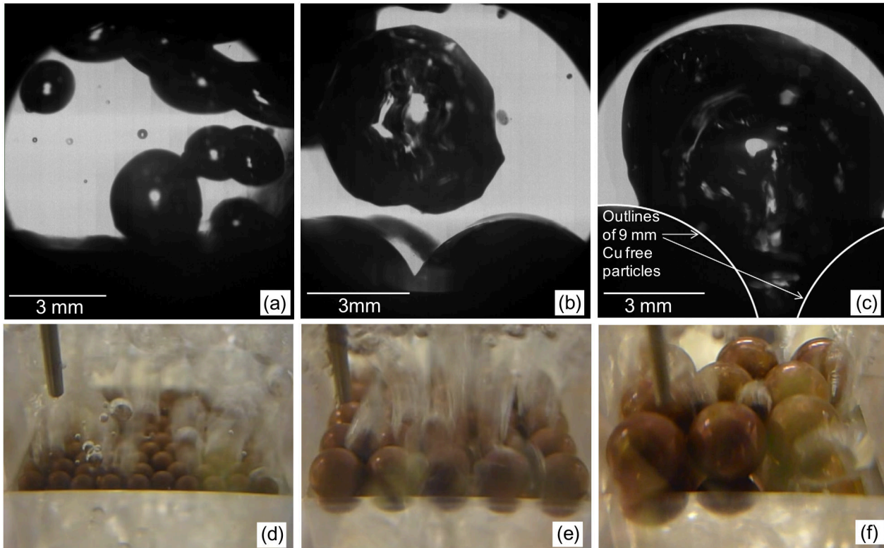
Fig. 5. High-speed microscopic visualization of the nucleate boiling characteristics for (a) one-hundred 3 mm particles at 77 kW/m 2 , (b) twenty-five 6 mm particles at 74 kW/m 2 , and (c) nine 9 mm particles at 75 kW/m 2 . Macroscopic views for the same respective cases are shown in (d), (e), and (f).
