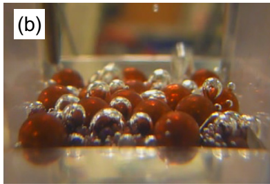
Fig. 7. A comparison of vapor bubble size at onset of nucleation boiling for (a) one-hundred 3 mm particles, (b) a mixture of fifty 3 mm particles and fifteen 6 mm particles, and (c) a microscopic view of case (a).
