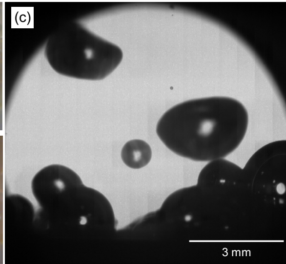
Fig. 7. A comparison of vapor bubble size at onset of nucleation boiling for (a) one-hundred 3 mm particles, (b) a mixture of fifty 3 mm particles and fifteen 6 mm particles, and (c) a microscopic view of case (a).
