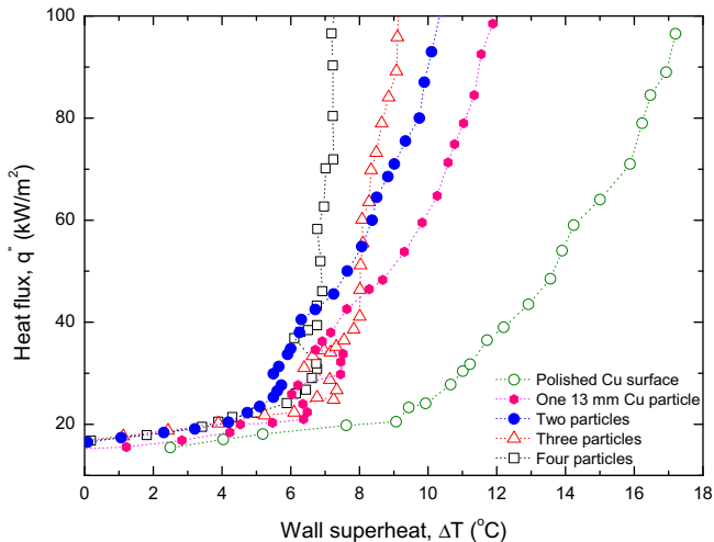
Fig. A1. Boiling curve showing the effect of number of 13 mm-diameter non-spherical free particles on boiling heat transfer.
